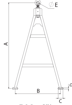
Tip 2 - Dereceli Okbaşı Type 2 - Towing Eye With Tube
